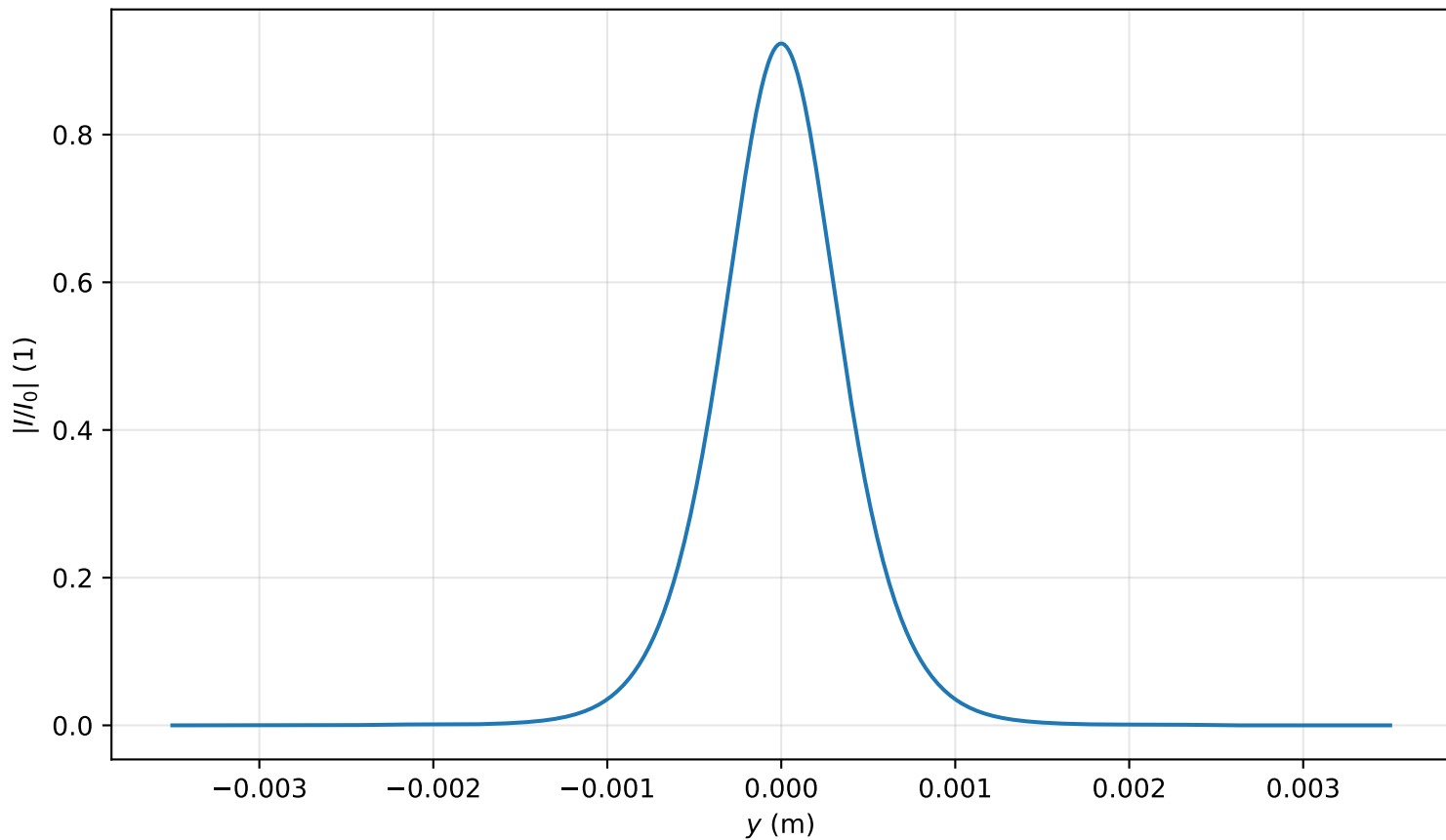
Intensity profile I(x=0, y, z=3.742)/I_0 , P_{in}=0.8P_{cr} , artificial time
